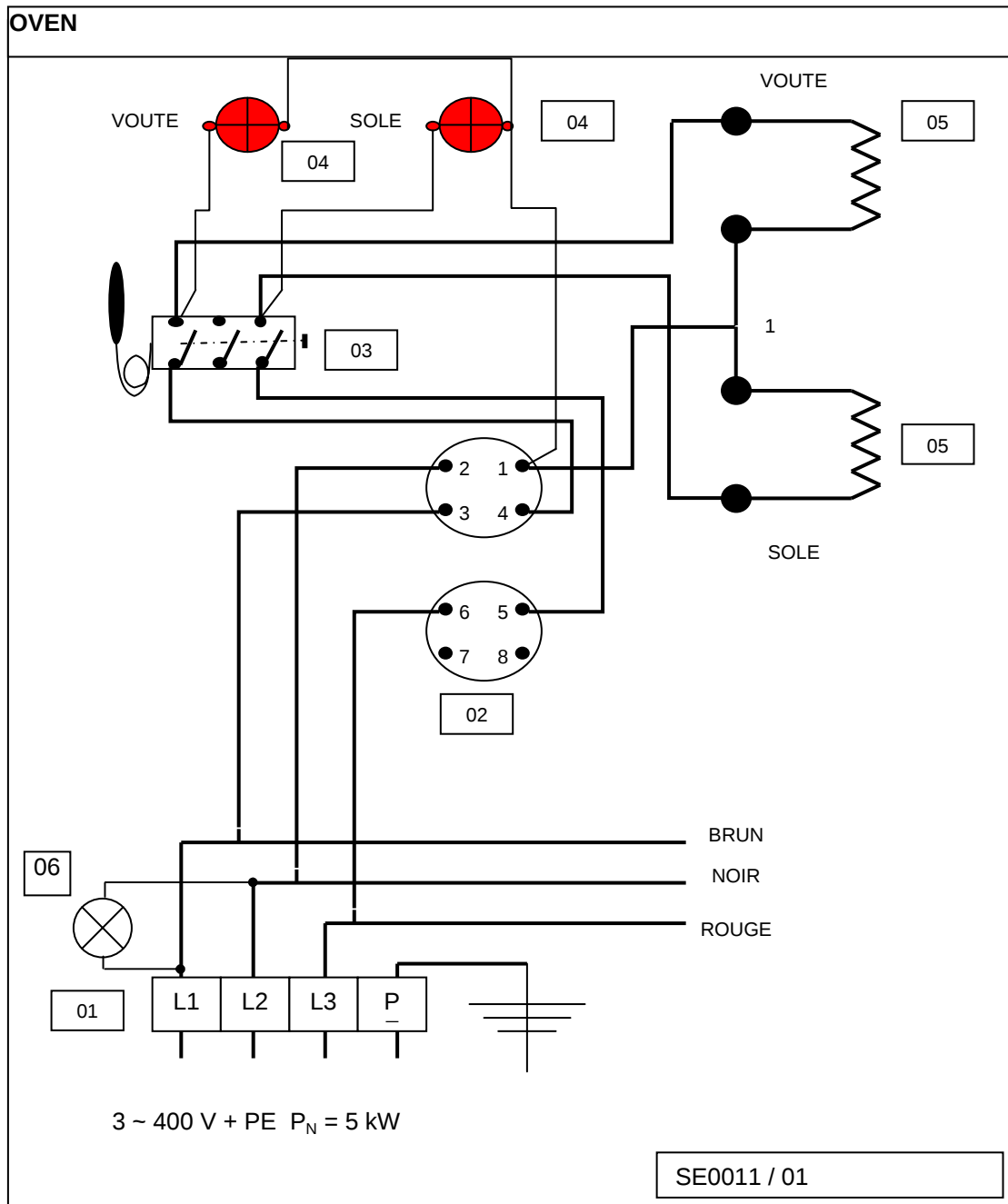
NOMENCLATURE: ELECTRIC OVEN 3~400 V (wiring diagram: SE0011 / 01)
