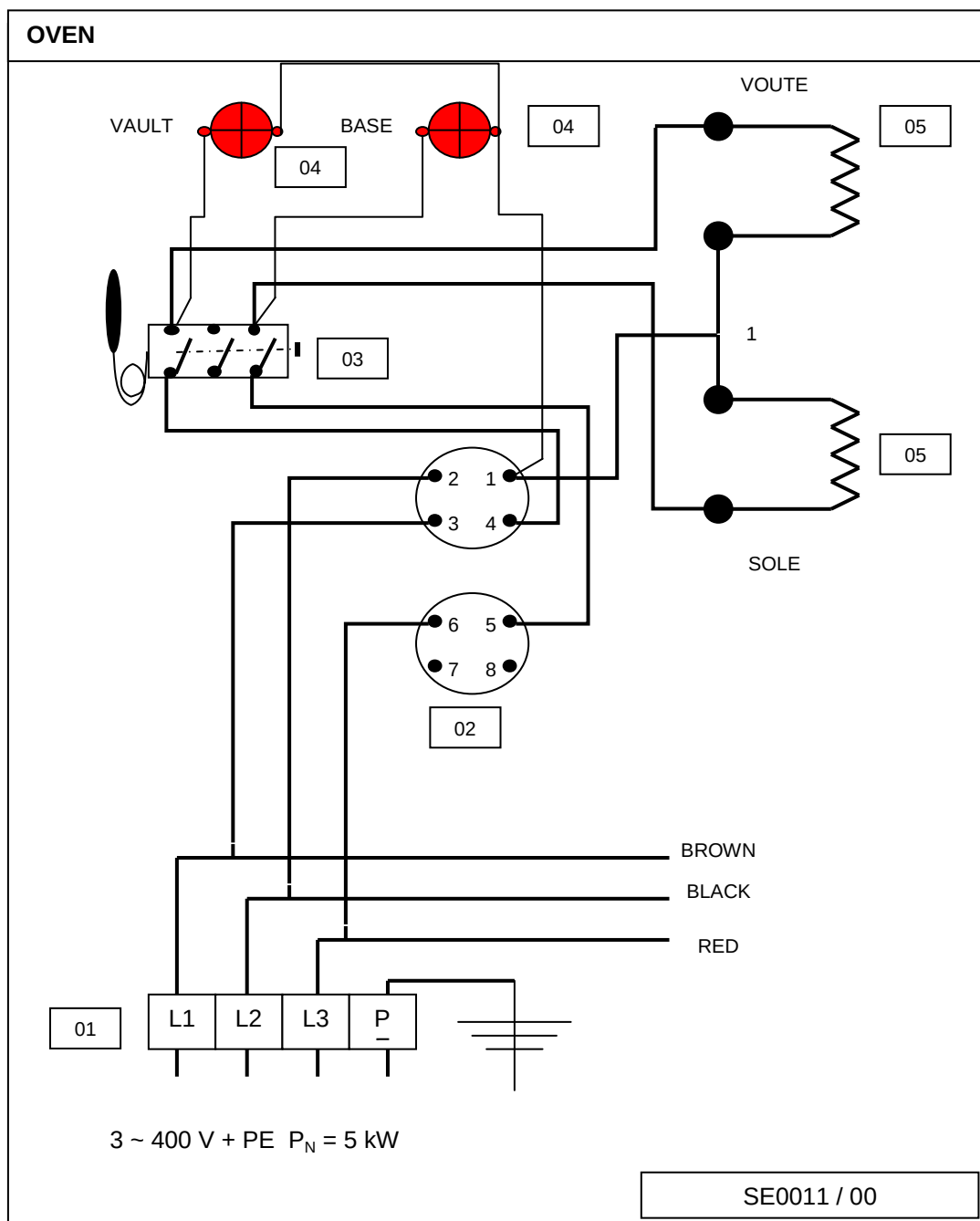
NOMENCLATURE: ELECTRIC OVEN (wiring diagram: SE0011 / 00)
